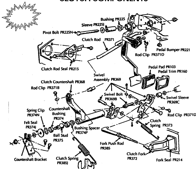
Typical 1969-72 GP Linkage
